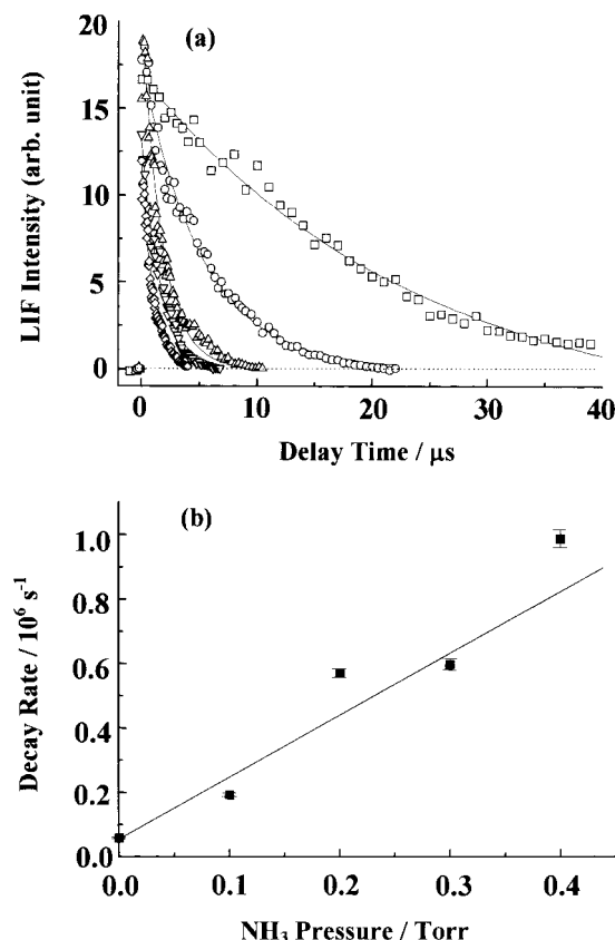
Fig. 3. (a) \text{NH}_3 addition effects on the transient LIF curves of \text{W}(\text{a } ^7\text{S}_3) at 6.0-Torr total pressure with Ar buffer gas. \text{NH}_3 pressures are 0.0 ( \square ), 0.1 ( \circ ), 0.2 ( \triangle ), 0.3 ( \nabla ), and 0.4 Torr ( \diamond ). Each solid line is a single-exponential decay fit obtained with an appropriate decay rate constant. (b) Determination of the apparent second-order depletion rate constant. Solid line is a linear fit.
